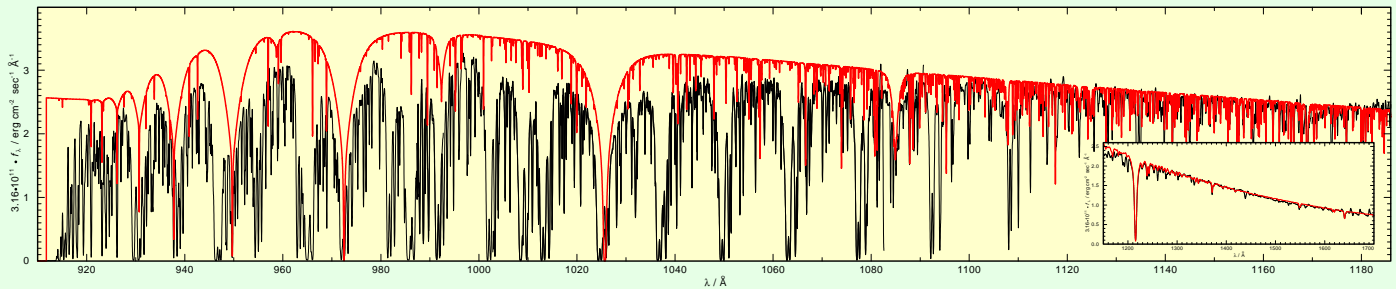
Fig. 1. FUSE observation of LSV+46°21 compared with a NLTE model-atmosphere spectrum which is normalized to match the flux level of a HST STIS observation (see the window on the right). The neutral hydrogen density is \log n_{\text{H I}} = 19.93 , and a reddening of E_{B-V} = 0.065 is applied. Note that the deviation between observation and photospheric spectrum is due to ISM line absorption.
