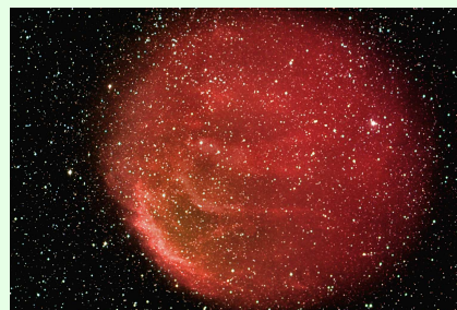
Fig. 2. Composite H \alpha (600 min, red) and [O III] 5007 Å (180 min, green) image of the PN Sharpless 2-216 (Dean Salman, www.galaxies.com).
