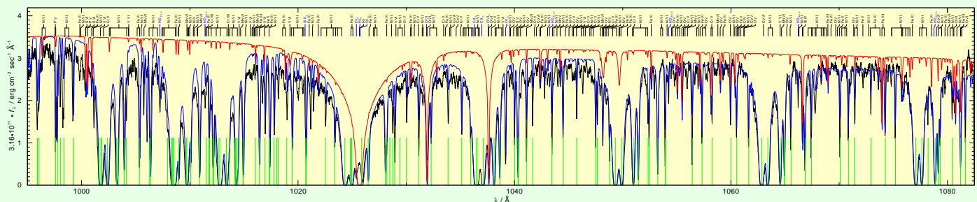
Fig. 4. Comparison of a section of the FUSE observation (black) with spectra of the pure photospheric model (red) and of the combined ISM + photospheric model (blue). Photospheric lines and interstellar lines are indicated at the top. The green marks at the bottom indicate interstellar H 2 absorption lines.
